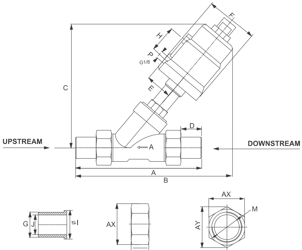
Male Threaded + Socket welded -- PV200S
